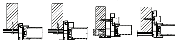
Vinyl with nail fin Vinyl with nail fin and J-channel Flush flange Box frame
