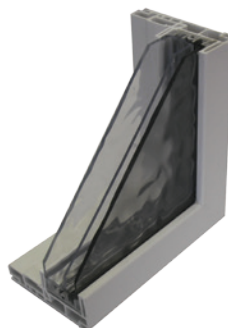
E3 SunBlock Cutaway Showing Triple Pane
