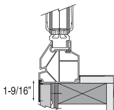
UV57 - Stucco Flange Snaps on exterior for use as exterior window trim.
