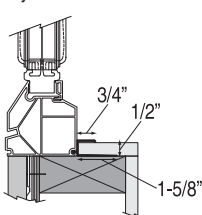
UV18 - Drywall Return Snaps on interior of frame. Provides channel for drywall.
