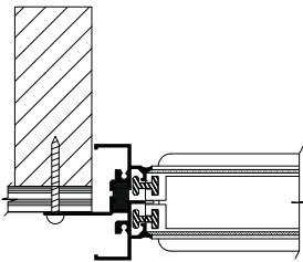
Aluminum 625/825 Fixed 7/8" Nail Fin Offset
