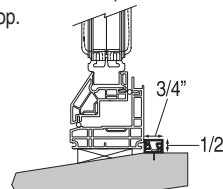
UV09 - Sill/Jamb Extender Finishes off the exterior gap where window sill meets opening sill. May also be used as jamb extender in some cases.
