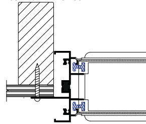
Aluminum 600/800 Fixed 7/8" Nail Fin Offset
