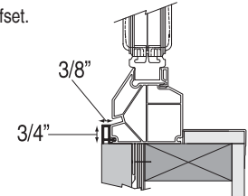
UV26 - Siding Return Snaps on exterior to cover gap where frame meets siding or other exterior finish. Must be field installed.
