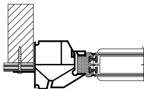
Vinyl Prestige II Fixed 7/8" Nail Fin Offset
