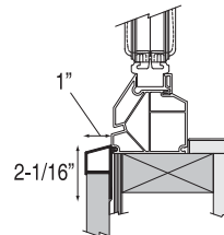
UV20 - Snap-In Brick Mold Snaps on exterior frame.
