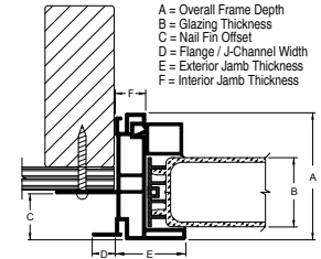
Vinyl Prestige II Casement & Awning 7/8" Nail Fin Offset
