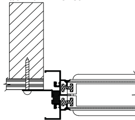
Aluminum 625/825 Fixed 1-3/8" Nail Fin Offset
