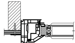
Vinyl Prestige II Casement & Awning 7/8" Nail Fin Offset
